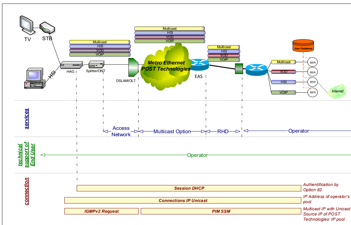
Figure 7: Multicast in Multi-VC configurations
