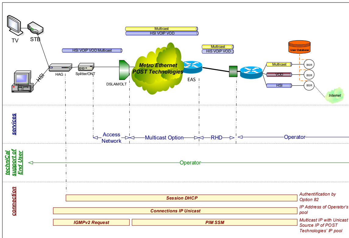
Figure 6: Multicast in Mono-VC configurations
