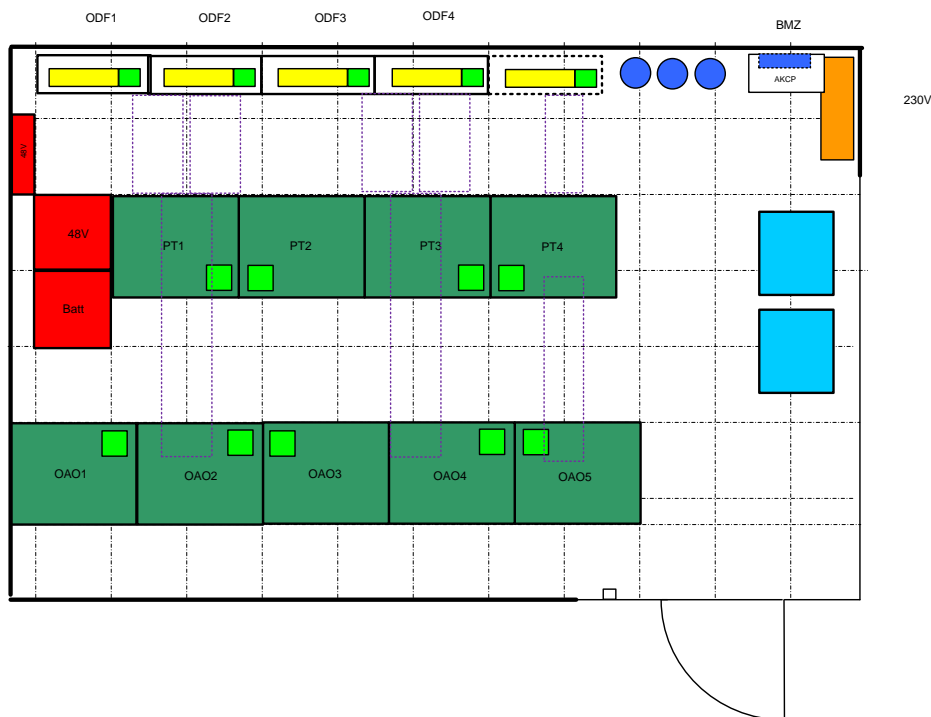
Figure 44 : Typical configuration of an Area POP
