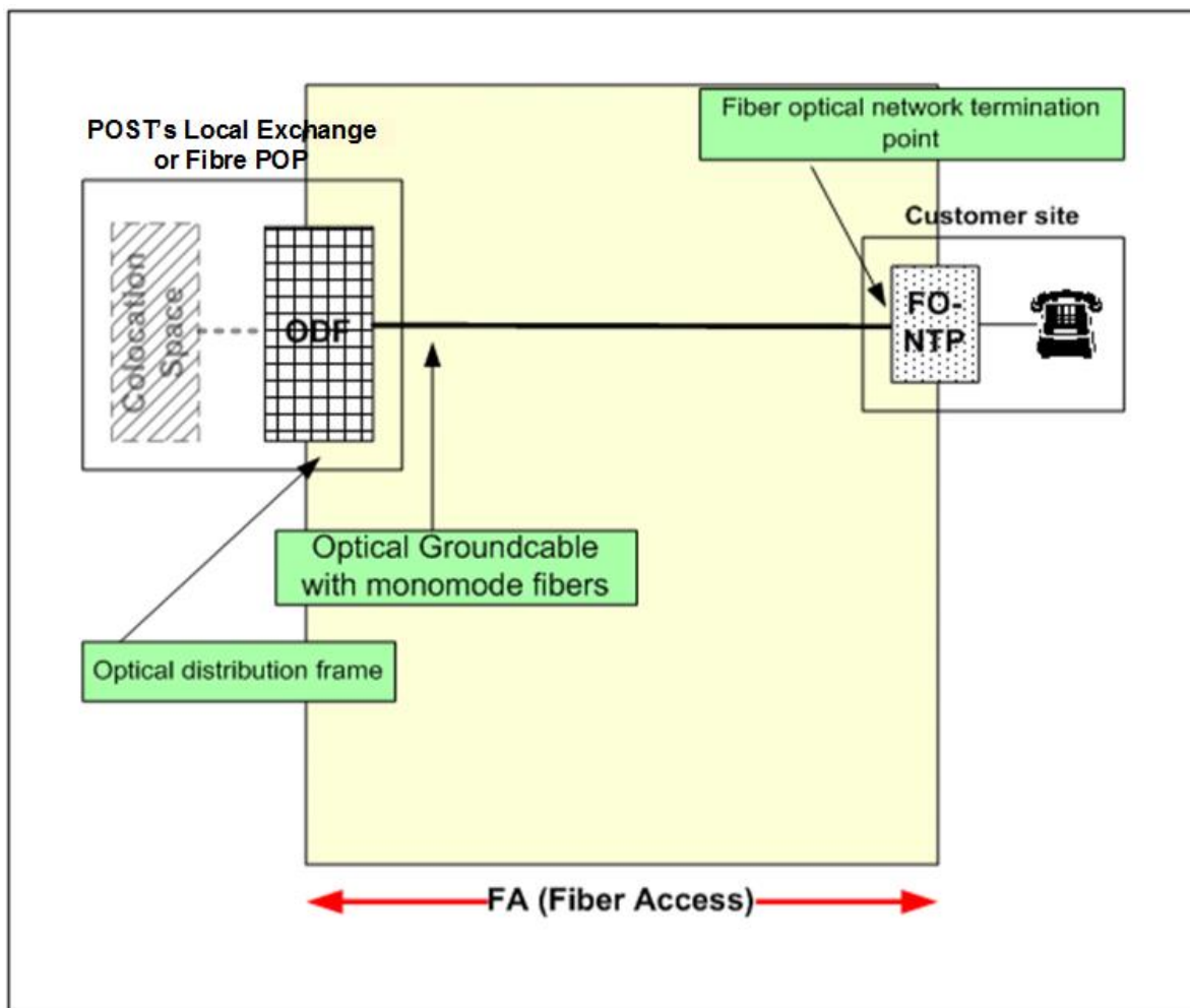
Figure 22 : FTTH Fibre Access (FA) Service in the point-to-point FTTH network
