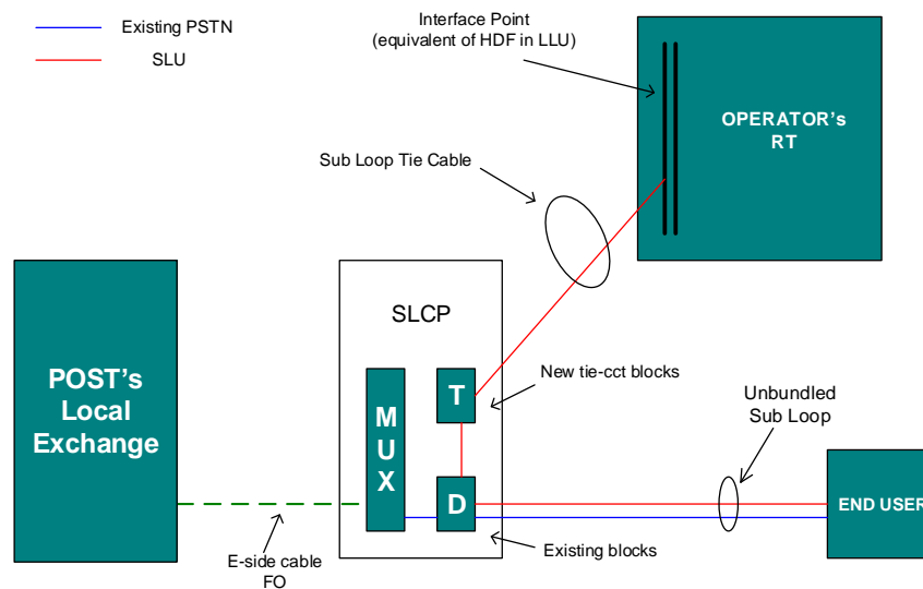
Figure 11 : Backhaul Connection of a Sub-Loop Connection Point (SLCP)
